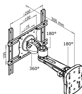
TILT &amp; SWING
