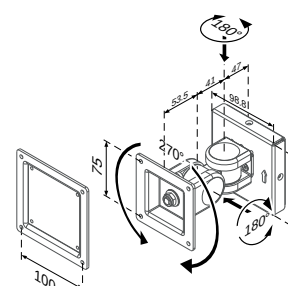
TILT &amp; SWING
